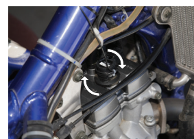
2/4 stroke install: Wrap pickup wire around head of coil
